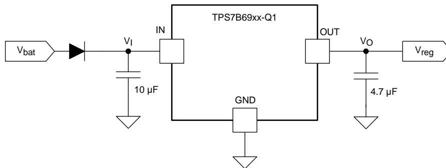
Figure 19. Typical Application Schematic for TPS7B69xx-Q1
